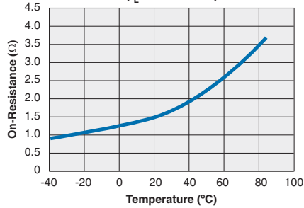
CPC1786 Typical On-Resistance vs. Temperature ( I_L=\text{max rated} )
