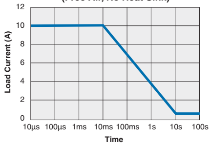
CPC1786 Energy Rating Curve (Free Air, No Heat Sink)
