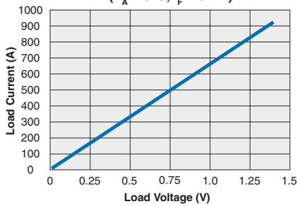
CPC1786 Typical Load Current vs. Load Voltage ( T_A=25^\circ\text{C} , I_F=10\text{mA} )
