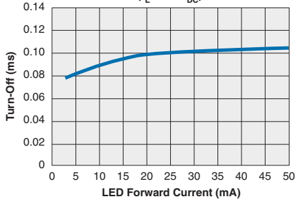
CPC1786 Typical Turn-Off vs. LED Forward Current ( I_L=0.5A_{DC} )
